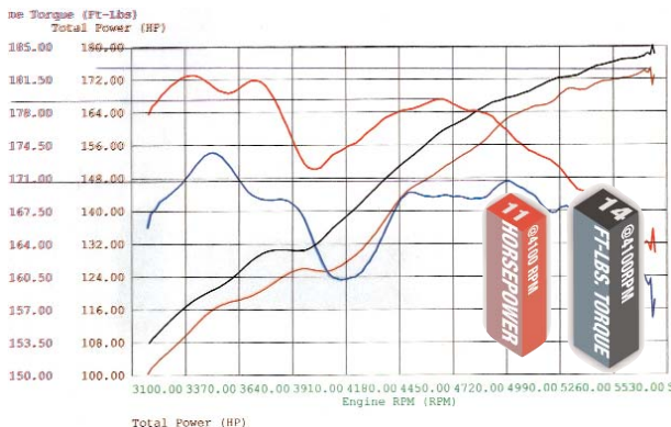
Dyno Results 54-10661 kit w/ performance exhaust and SMG.
