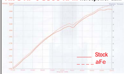
11.75 HP @ 5900 RPM Horsepower Gain
