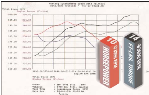
Dyno Results 1998 BMW 540i E39
