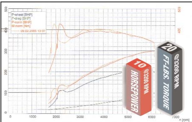
Dyno Results 2002 BMW X5 (E53)
